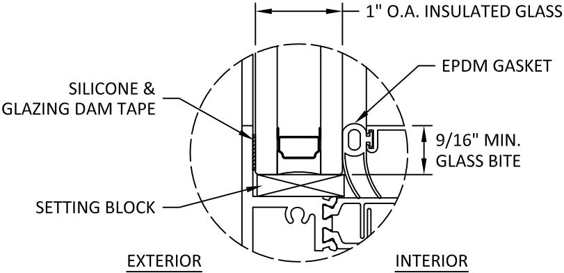
GLAZING DETAIL
