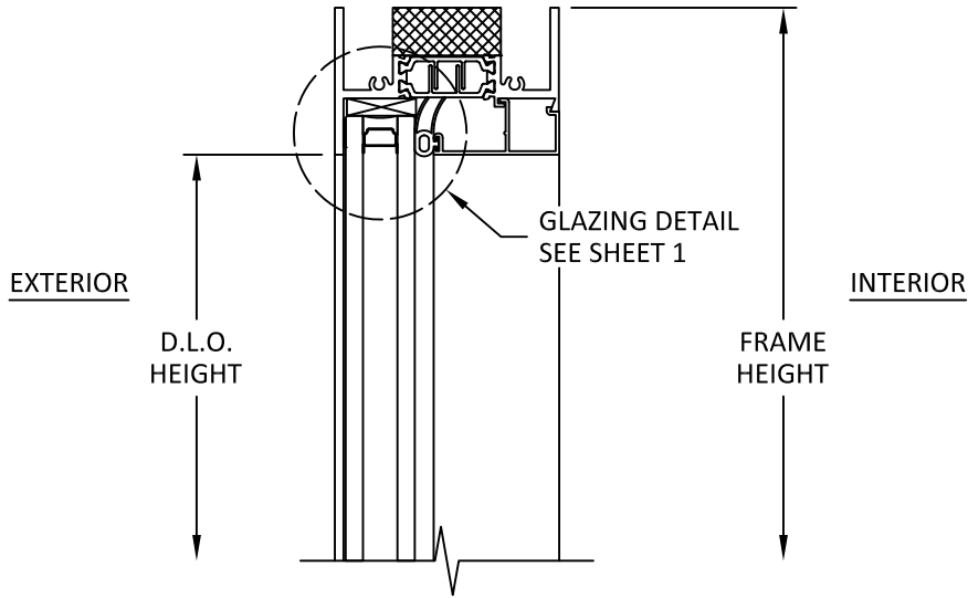
A 3 VERTICAL SECTION HEAD
